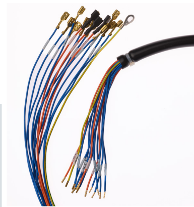
Multi-core cable with crimped fastons and cable lug. The other side is labeled.
