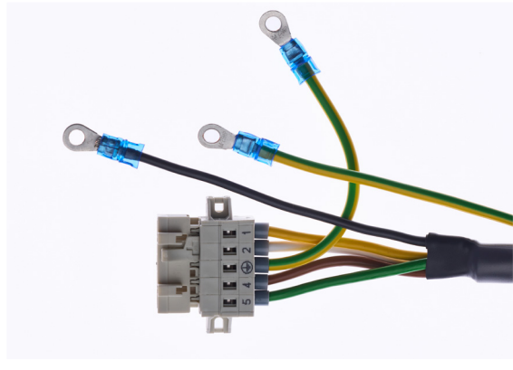
Multicore cable – ferrules crimped onto the cores, connector assembled, and additional cores fitted with crimped cable lugs.
