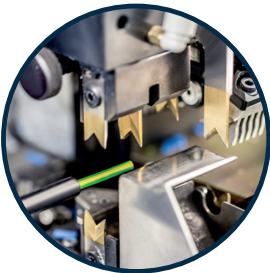
CUTTING
