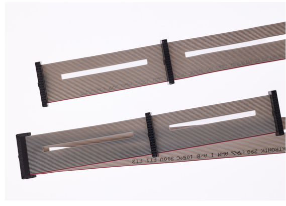
Flat cable with crimped connectors and cut sections.
